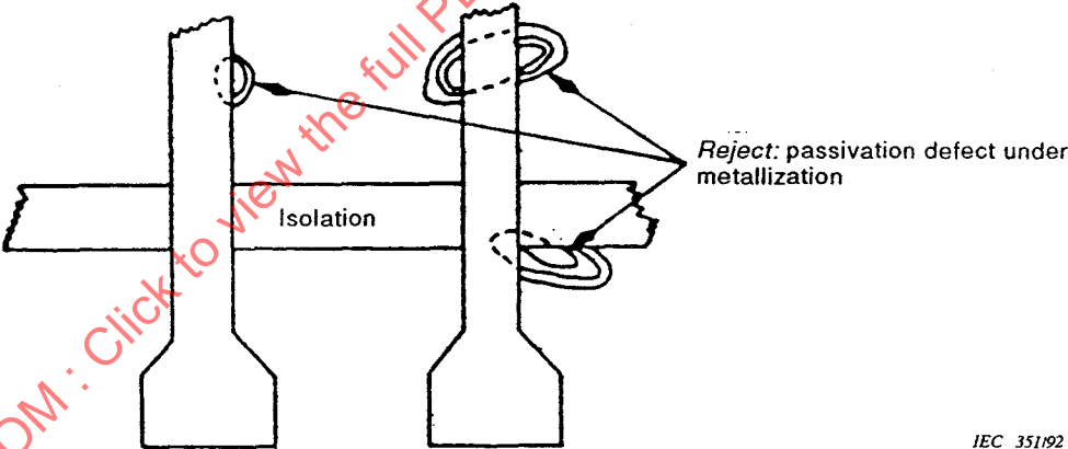
Figure 10 – Passivation faults
