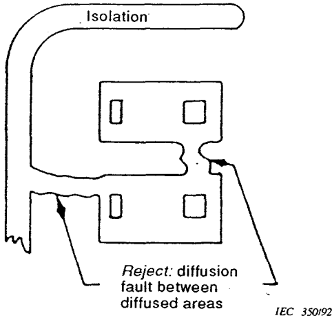
Figure 9 – Diffusion faults
