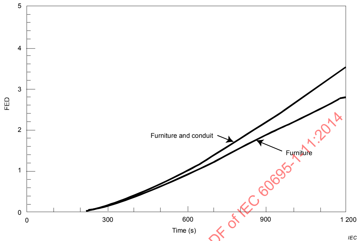
Figure B.9 – Relative increase of toxicity due to exposed conduit (gypsum wall board)
