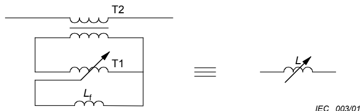
Figure 3 – Arrangement to produce the variable inductor L in figure 2
