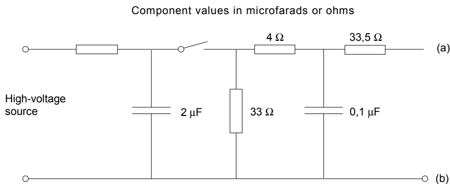
Figure 7 – Pulse generator 1,2/50
