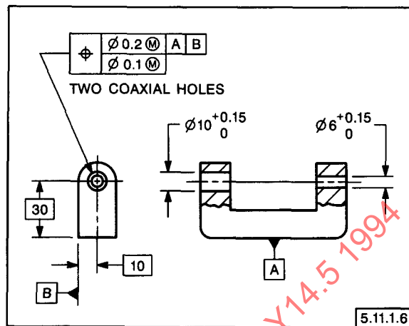
FIG. 5-53 POSITIONAL TOLERANCING FOR COAXIAL HOLES OF DIFFERENT SIZE
