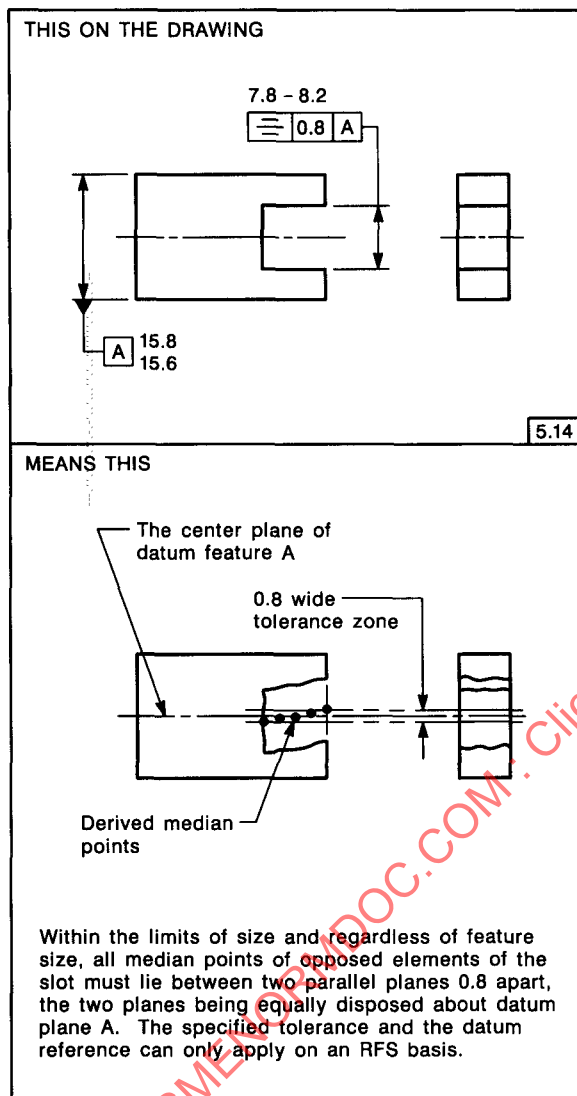
FIG. 5-61 SYMMETRY TOLERANCING
