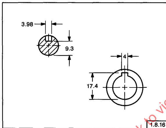
FIG. 1-45 KEYSEATS
