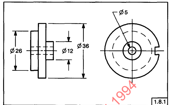
FIG. 1-19 DIAMETERS
