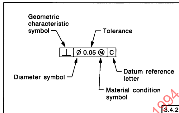
FIG. 3-20 FEATURE CONTROL FRAME INCORPORATING A DATUM REFERENCE
