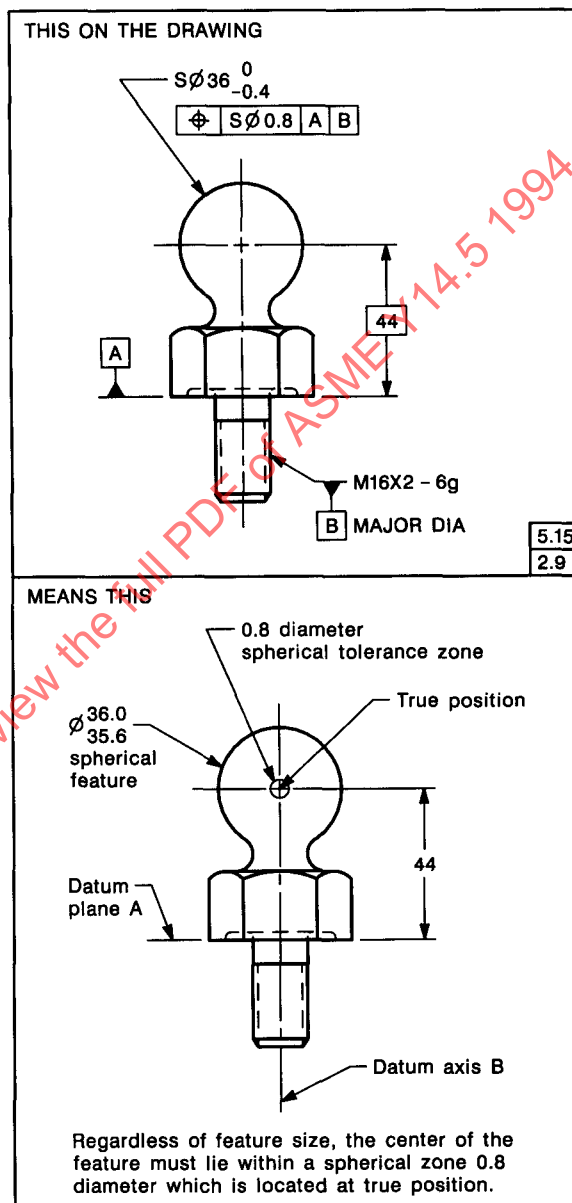
FIG. 5-62 SPHERICAL FEATURE LOCATED BY POSITIONAL TOLERANCING
