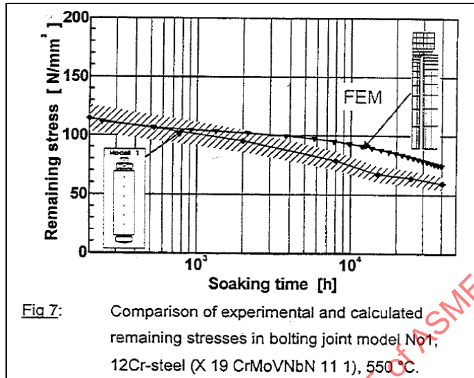
Figure 15 – FEA Bolt Load Relaxation Results from Maile, et. al. [18], Fig. 7, page 156
