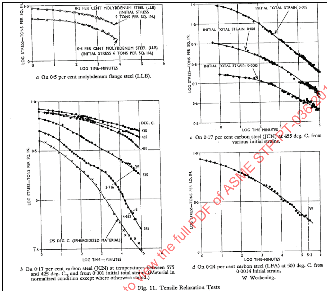
Figure 8 – Flange Ring Relaxation Graphs from Johnson [11], Fig. 11, page 432
