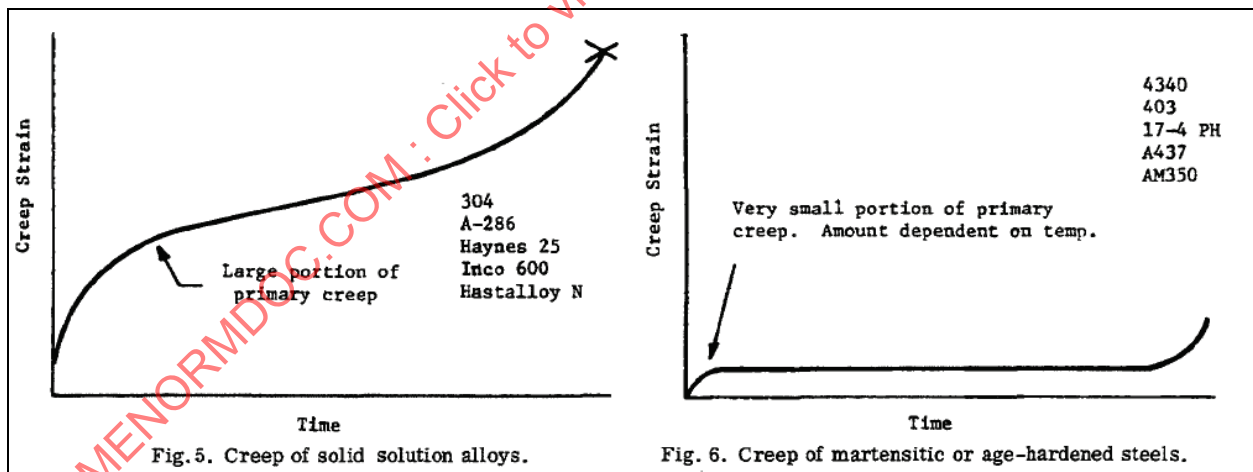
Figure 13 – Creep Characteristics of Different Materials from Cooper, et. al. [14], Fig. 5 to Fig.7, page 133
