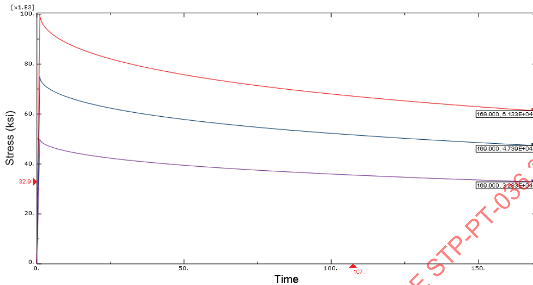
Figure 36 – Bolt/Cylinder Full FEA Model Bolt Stress vs. Time Results
