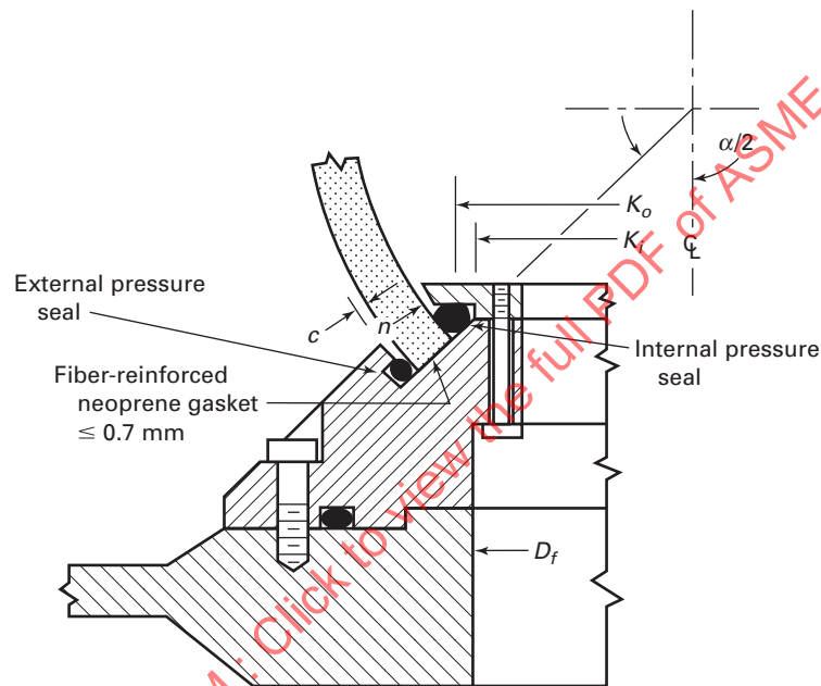
Fig. 2-2.10.1-6 Seat Cavity Requirements — Hyperhemispherical Window
