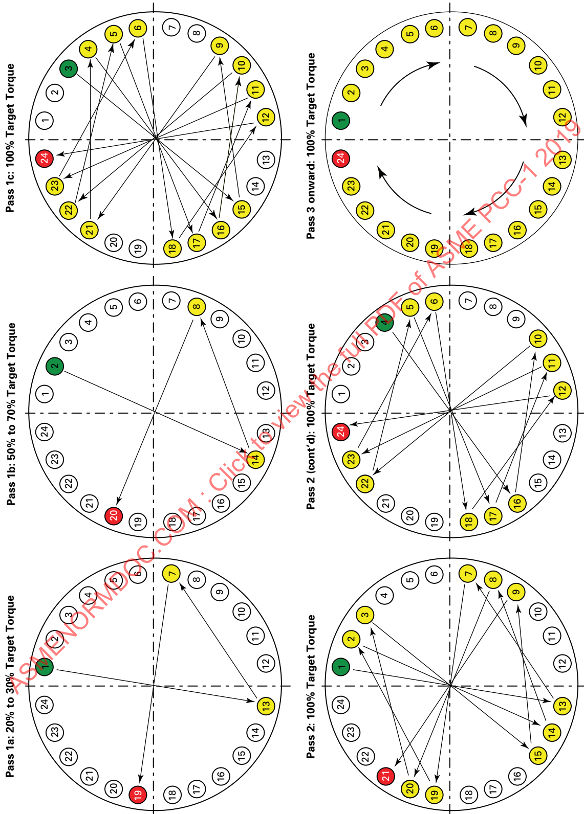
Figure F-8 Alternative Pattern #2A: Quadrant Pattern: Star Sequencing (Single Tool)
