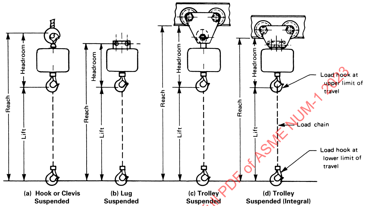
Figure GR-6.2.7.1-3 Electric- and Air-Operated Chain Hoist Suspension Types
