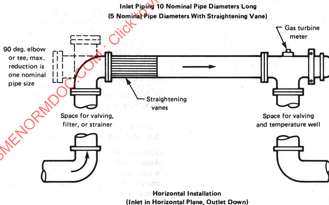
FIG. 5 RECOMMENDED INSTALLATION OF AN ANGLE BODY GAS TURBINE METER (MINIMUM LENGTHS)
