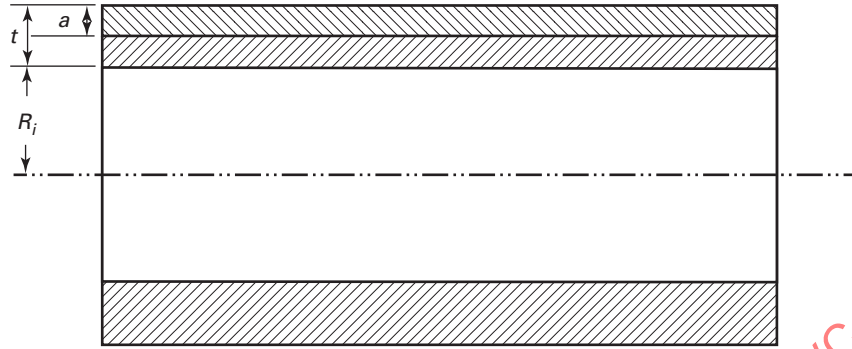
Figure A-3561-1 Axial Outside Surface Flaw With a/\ell = 0 in a Cylinder
