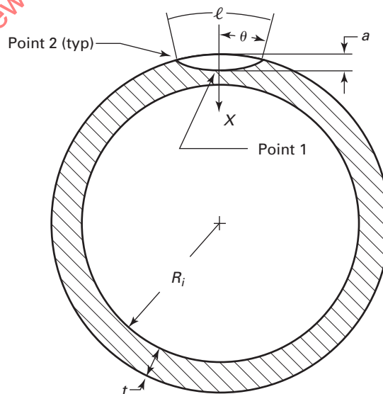
Figure A-3540-1 Cylindrical Semielliptical Outside Surface Flaw Geometry
