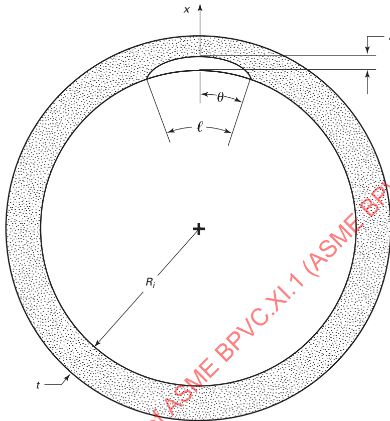
Figure A-3530-1 Cylindrical Flow Geometry
