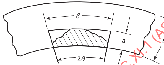
(b) Surface Flaw (Inner)
