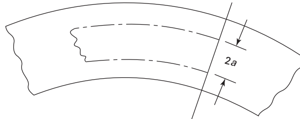
Figure C-2400-1 Flaw Characterization — Skewed Axial Flaws Projected Into Axial Plane
