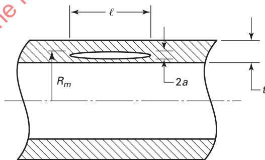
Figure C-4310-4 Axial Subsurface Flow Geometry
