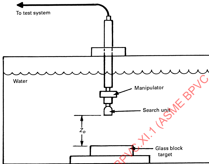
Figure VIII-S1-1B Test Configuration
