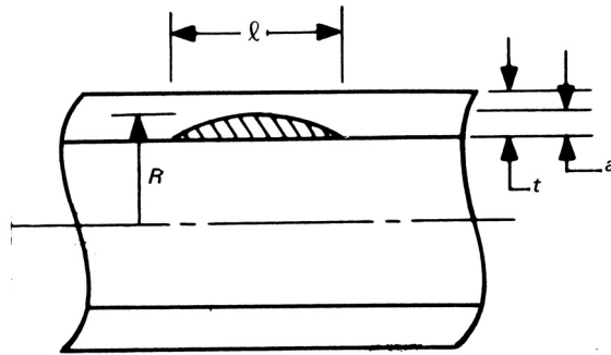
Figure H-4400-2 Axial Flaw Geometry
