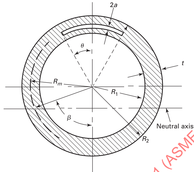
Figure C-4310-3 Circumferential Subsurface Flow Geometry
