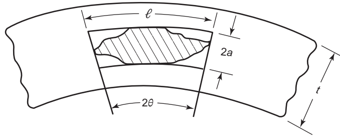
(a) Subsurface Flaw
