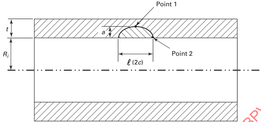
Figure A-3550-1 Axial Inside Surface Flaw in a Cylinder
