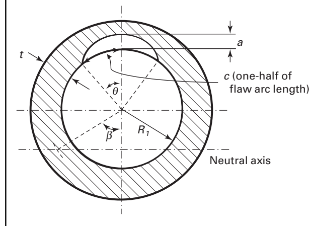
Figure C-4310-5 Semielliptical Circumferential Inside Surface Flaw Geometry
