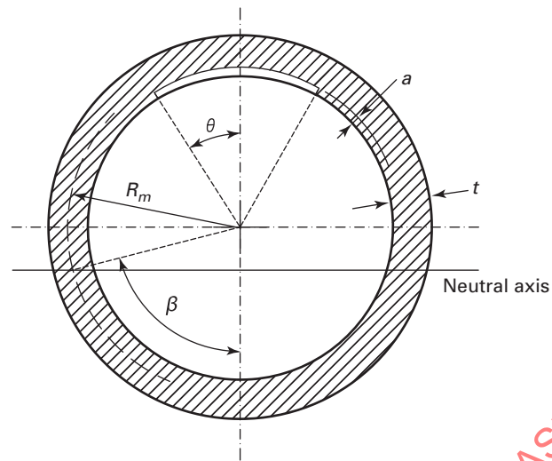
Figure C-4310-1 Circumferential Surface Flaw Geometry
