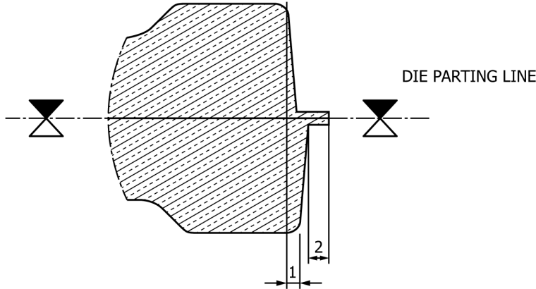
FIG. X2.4 Flash Projection
