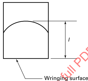
Figure 10.5.1-1 Half-Round Jaw
