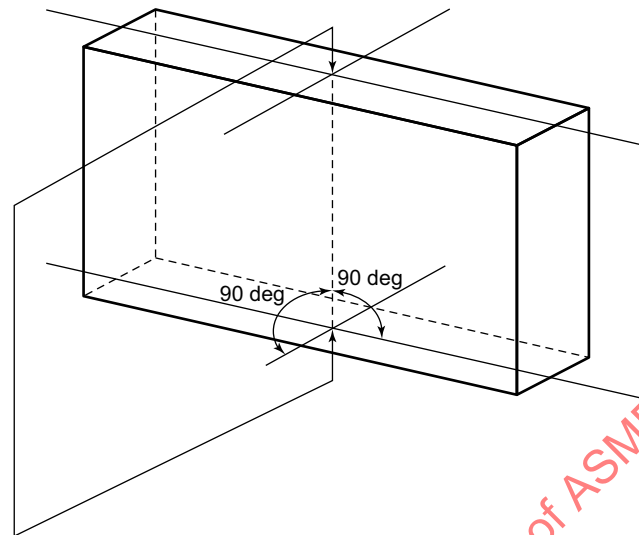
Figure 9.4.1-1 Measurement of Gage Length by Comparison Taking the Perpendicular Distance From the Reference Point of a Measuring Face to the Opposite Face
