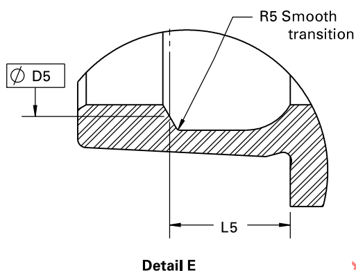
NOTES: 1. Refer to Table 1-4-1 for dimension values. 2. The texture is per ASME B46.1. Unless otherwise specified, surface texture, R_a , is 3.2 \mu\text{m} . 3. All sharp edges.
