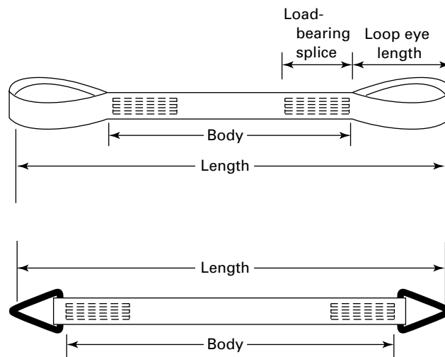
Fig. 9-5.0-2 Synthetic Webbing Sling Nomenclature
