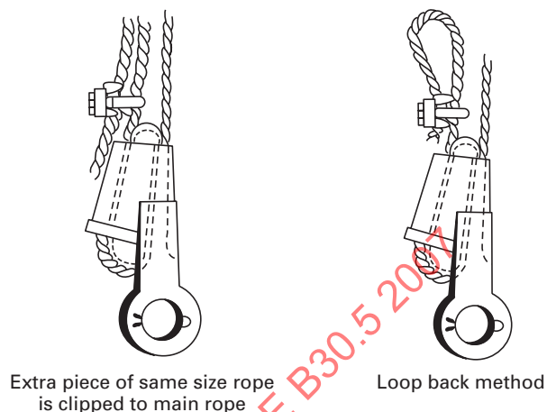
Fig. 14 Dead Ending Rope in a Socket
