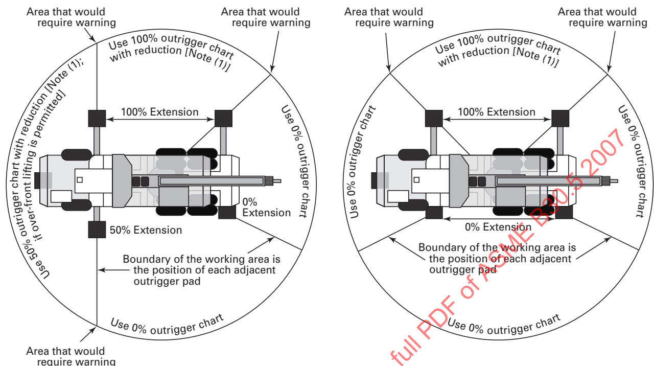
Fig. 16 Examples of Typical Unequal Outrigger Extension Positions
