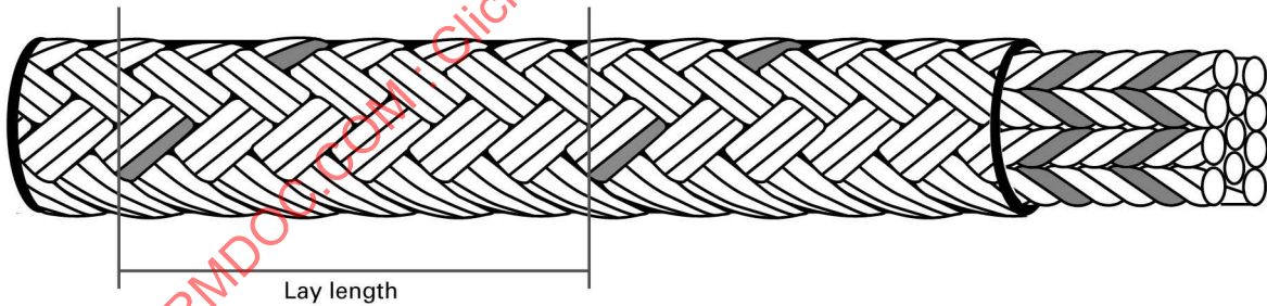
Figure 30-2.3.1-4 Parallel Core, Braided Jacket: Three-Strand Cores
