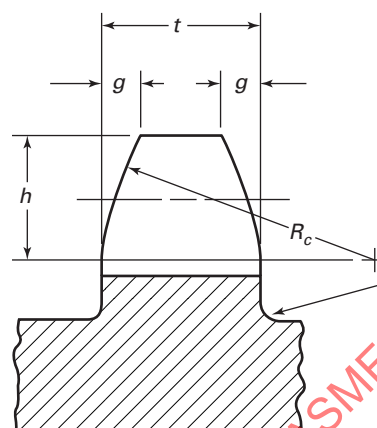
Section B
