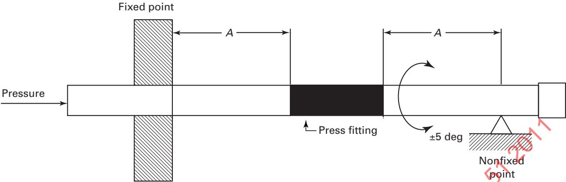
Fig. 9 Test Setup for Dynamic Torque Test
