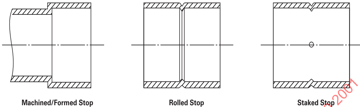
FIG. 2 TUBE STOPS
