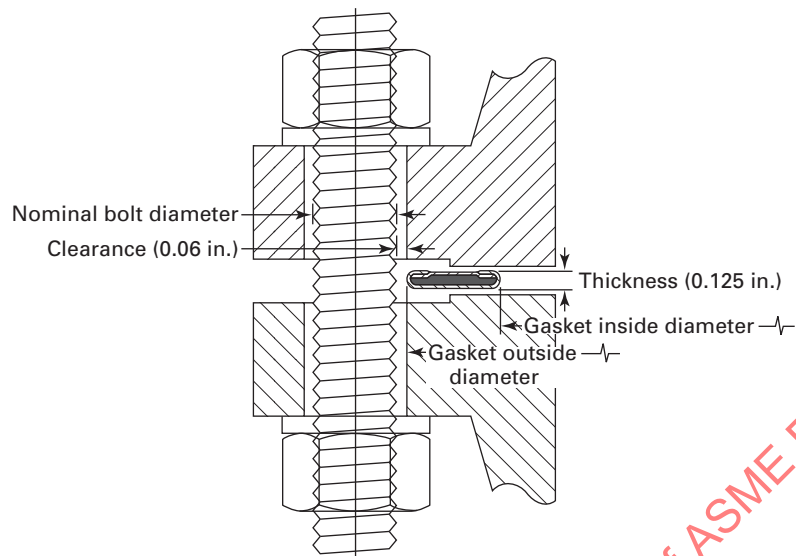
Fig. I-2 Jacketed Gaskets (U.S. Customary)
