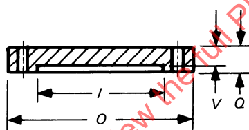
NPS 10 and Smaller Blind Flange
