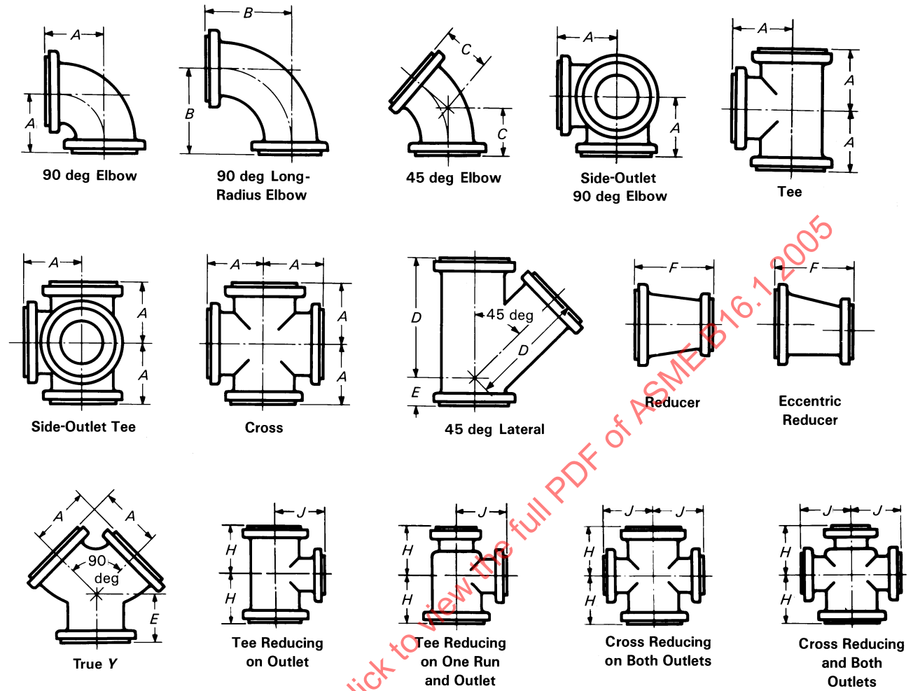
Fig. I-7 Class 250 Flanged Fittings
