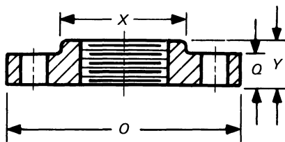
Fig. I-2 Class 25 Flange
