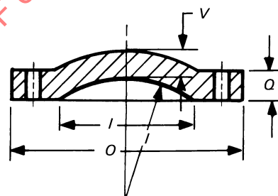
NPS 12 and Larger Blind Flange
