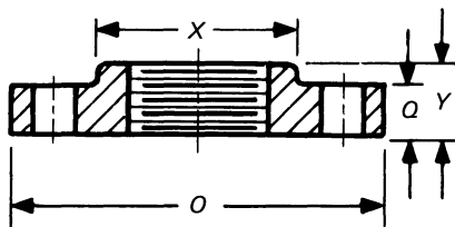
Fig. 2 Class 25 Flanges
