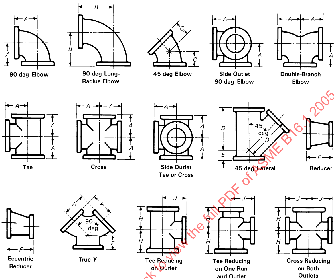
Fig. 5 Class 125 Flanged Fittings
