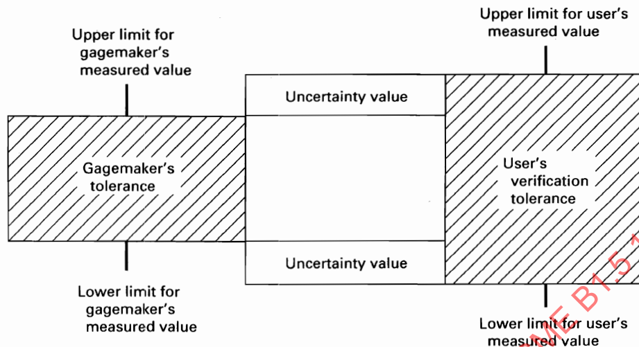
FIG. 6 GAGE ACCEPTANCE USING MEASUREMENT UNCERTAINTY
