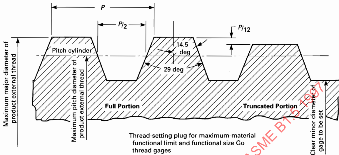
FIG. 9 GO THREAD FORM — FULL-FORM AND TRUNCATED SETTING PLUG GAGE FOR EXTERNAL THREAD
