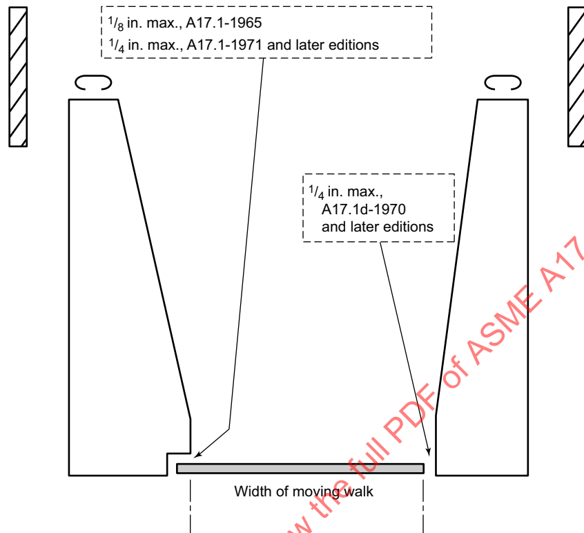
Figure 9.15.1-1 Treadway Clearances
