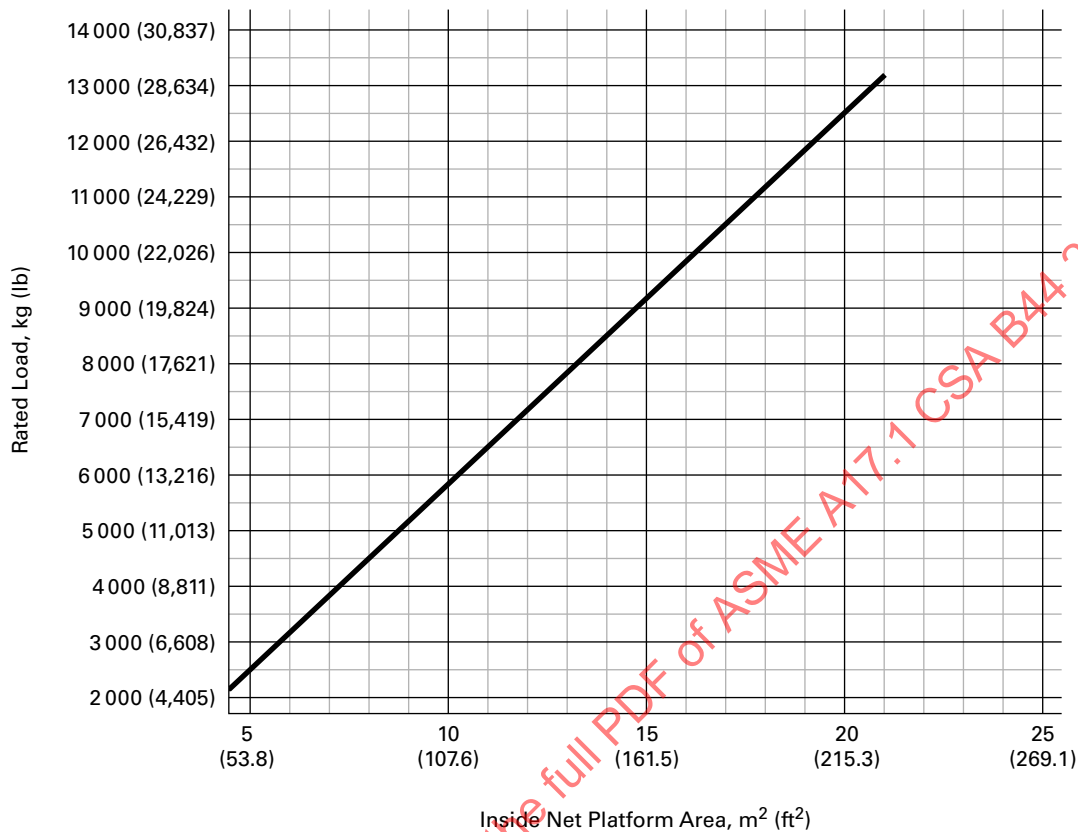
Figure 8.2.1.2 Minimum Rated Load for Passenger Elevators (Cont'd)
