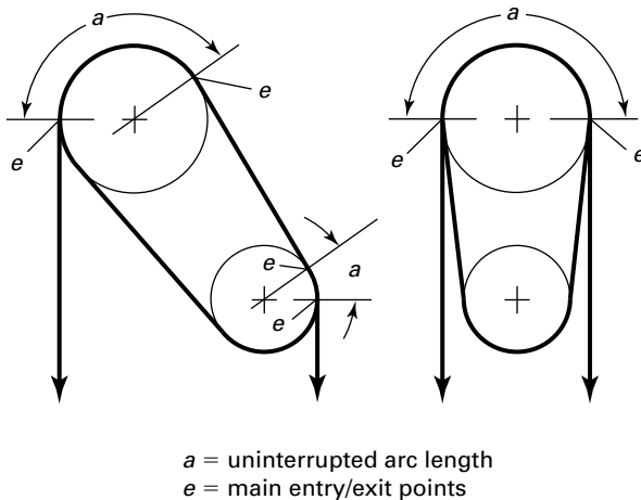
Figure 8.4.3.1.3 Arc of Contact
