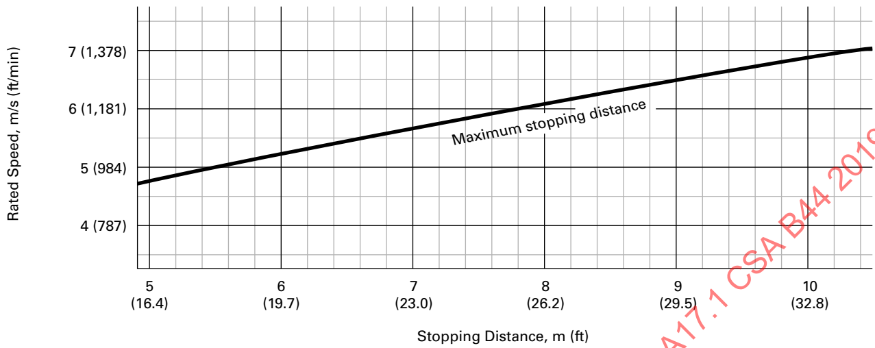
Figure 8.2.6 Stopping Distances for Type B Car and Counterweight Safeties (Cont'd)
