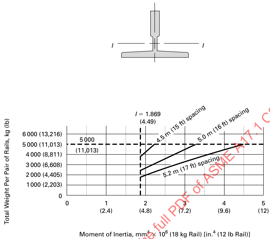
Figure 2.23.4.1-2 Minimum Moment of Inertia About x-x Axis for a Single Guide Rail With Its Reinforcement (Cont'd)
