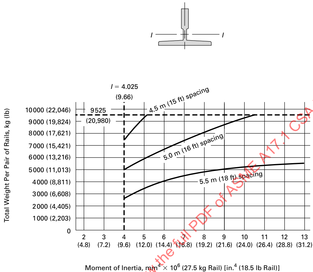
Figure 2.23.4.1-2 Minimum Moment of Inertia About x-x Axis for a Single Guide Rail With Its Reinforcement (Cont'd)
