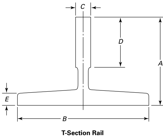
Figure 2.23.3 Elevator Guide Rails
